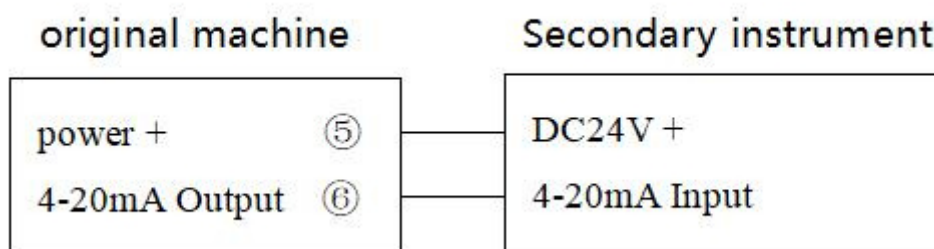
Schematic diagram of the connection of two-wire
